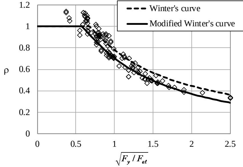
Figure 4. Chart. Comparison of experimental test resistances from welded stub column test data collected and generated by Schillo (2017) to Winter's classical effective width equation and to the modified form of this equation recommended in this research.
