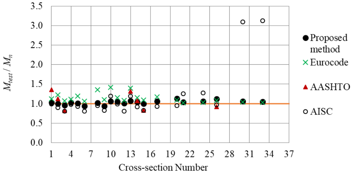
Figure 6. Chart. Comparison of nominal strength estimates to strengths from test simulation for homogeneous welded box-section members with L_b \approx (0.5L_p + L_{max})/2 .
