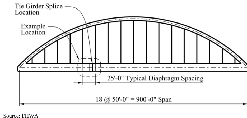
Figure 41. Illustration. Tied arch elevation.
