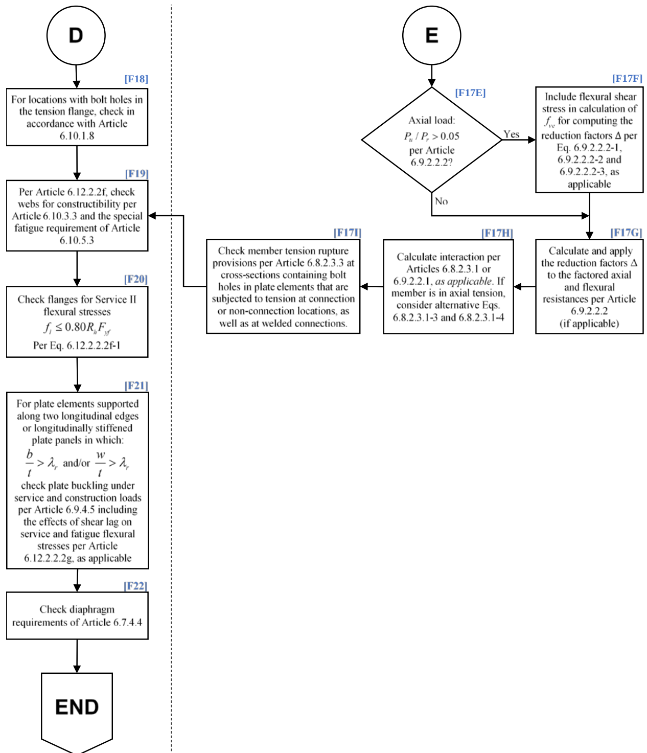
Figure 36. Figure C6.5.2-1—flowchart for LRFD Article 6.12.2.2—flexural resistance of rectangular noncomposite box-section members (continued).
