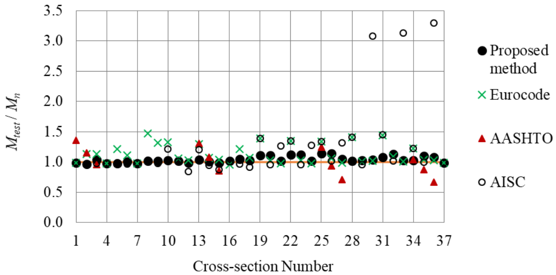
Figure 5. Chart. Comparison of nominal strength estimates to strengths from test simulation for homogeneous welded box-section members with L_b \approx 0.5L_p .
